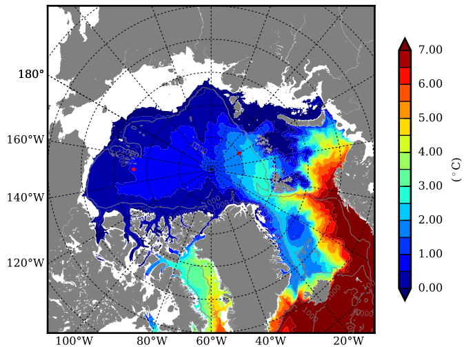
REF02 AW Max Temp over 2013
