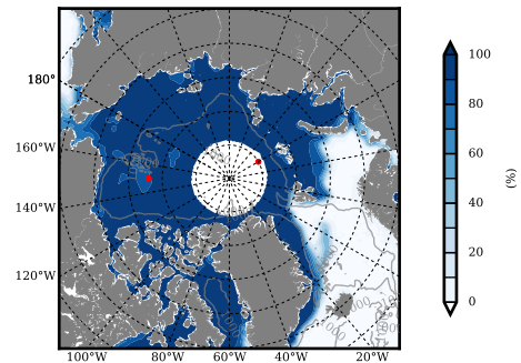
NSIDC mean SICON m09 1988
