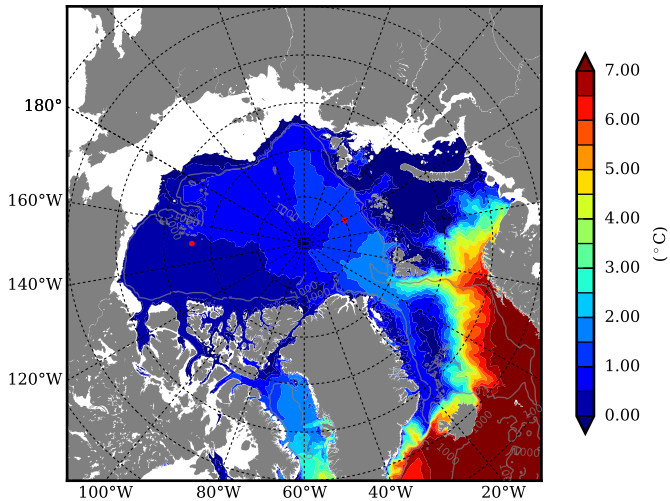
REF03 AW Max Temp over 1980
