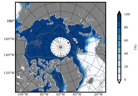
NSIDC mean SICON m09 1980
