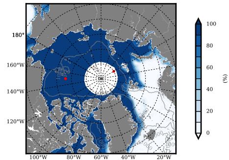
NSIDC mean SICON m09 1991
