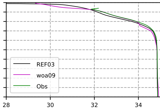
1996 mean Salinity @ moor Arctic B box
