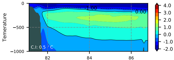
REF03 / Kara Section 1980
