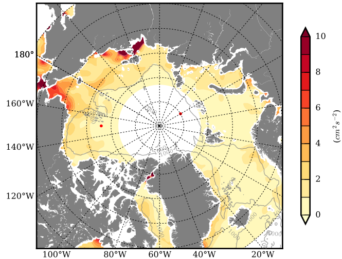
mean PSI over 2005
