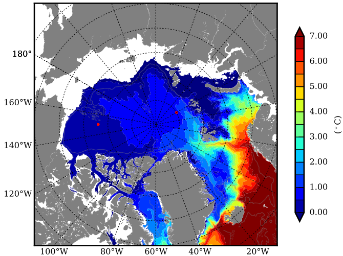
REF06 AW Max Temp over 1984
