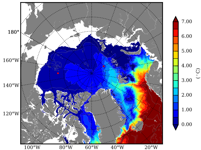
REF06 AW Max Temp over 1988
