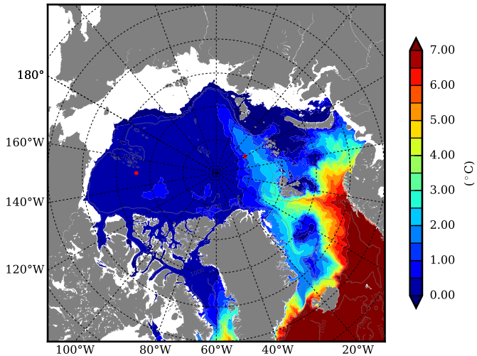
REF06 AW Max Temp over 1996
