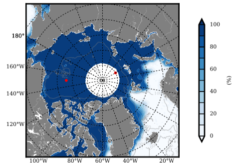
NSIDC mean SICON m09 1979
