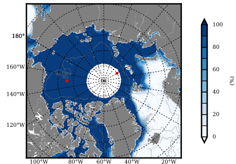
NSIDC mean SICON m09 1992
