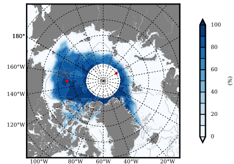
NSIDC mean SICON m09 1994
