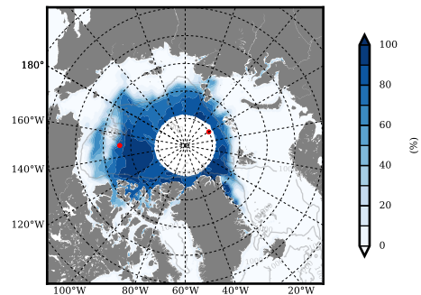
NSIDC mean SICON m09 2005
