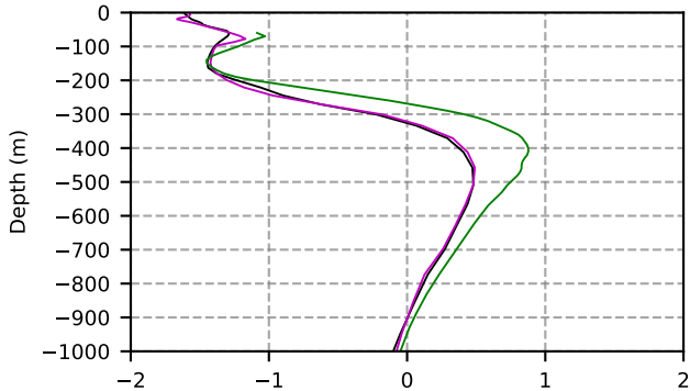
1981 mean temperature @ moor Arctic B box
