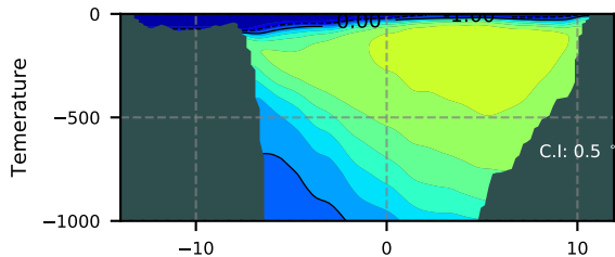
REF06 / FramS Section 1987
