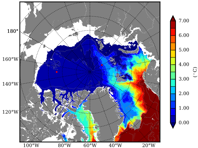
REF07 AW Max Temp over 2007
