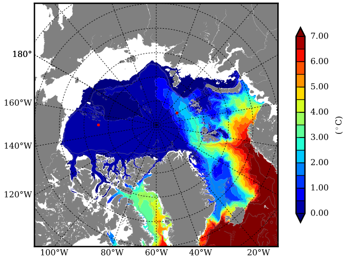
REF07 AW Max Temp over 2012
