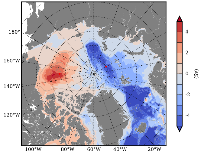
mean PSI over 2003
