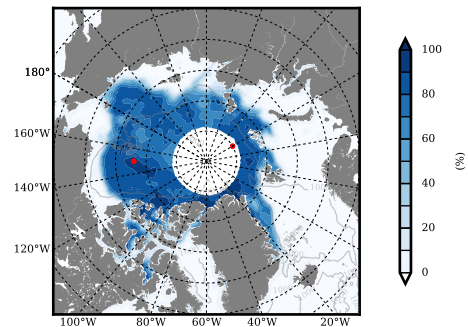
NSIDC mean SICON m09 1981
