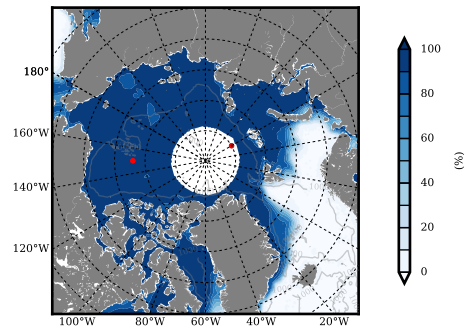
NSIDC mean SICON m09 1985
