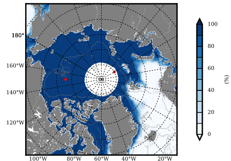
NSIDC mean SICON m09 1990
