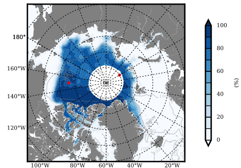
NSIDC mean SICON m09 1996
