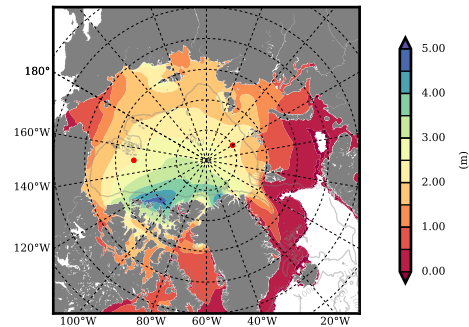
NSIDC mean SICON m03 1996
