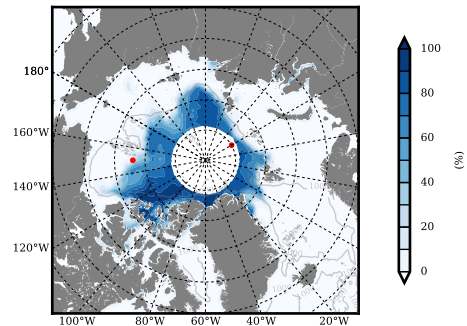
NSIDC mean SICON m09 2007
