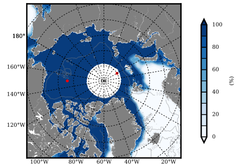
NSIDC mean SICON m09 2009
