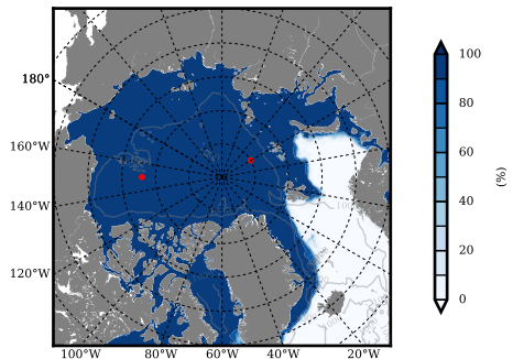
mean SICON m09
