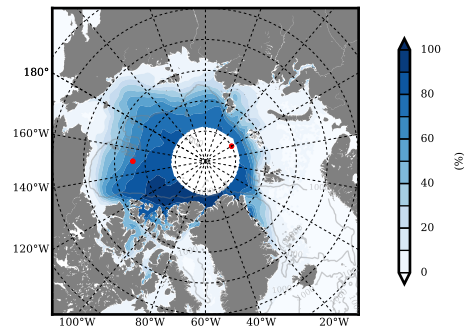
NSIDC mean SICON m09 2015
