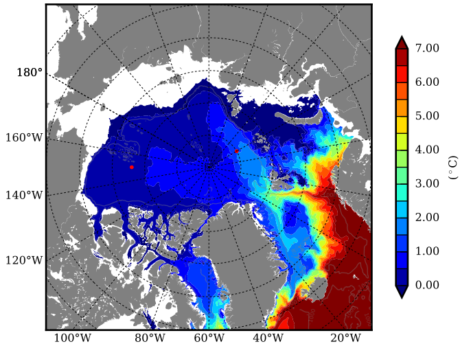
REF08 AW Max Temp over 1989
