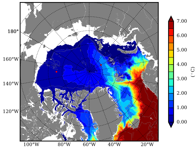
REF08 AW Max Temp over 1990
