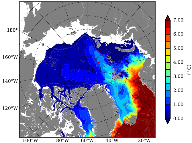
REF08 AW Max Temp over 1991
