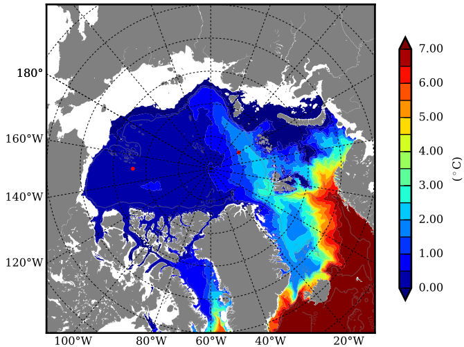
REF08 AW Max Temp over 1996
