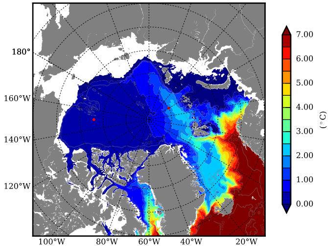
REF08 AW Max Temp over 1998
