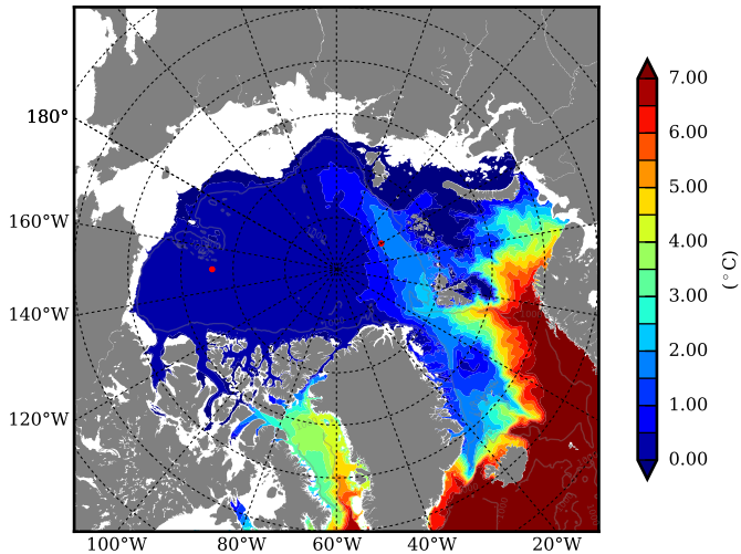
REF08 AW Max Temp over 2008
