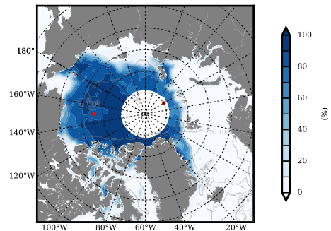
NSIDC mean SICON m09 1982
