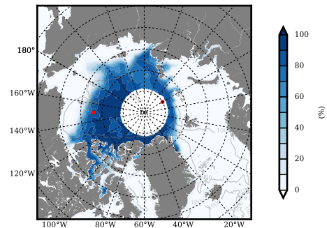
NSIDC mean SICON m09 2003
