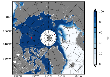
NSIDC mean SICON m09 2011
