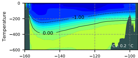
REF08 / Beaufort Section 2011
