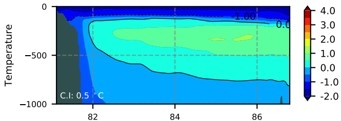
REF08 / Kara Section 1982
