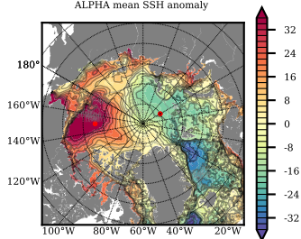
ALPHA mean SSH anomaly
