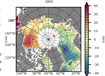
Mean DOT from Armitage et al. 2017 2004
