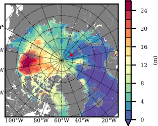
Mean FWC (m) from Init State
