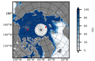
NSIDC mean SICON m09 2003
