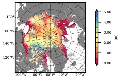
mean SICON m03
