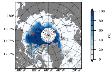
NSIDC mean SICON m09 2004
